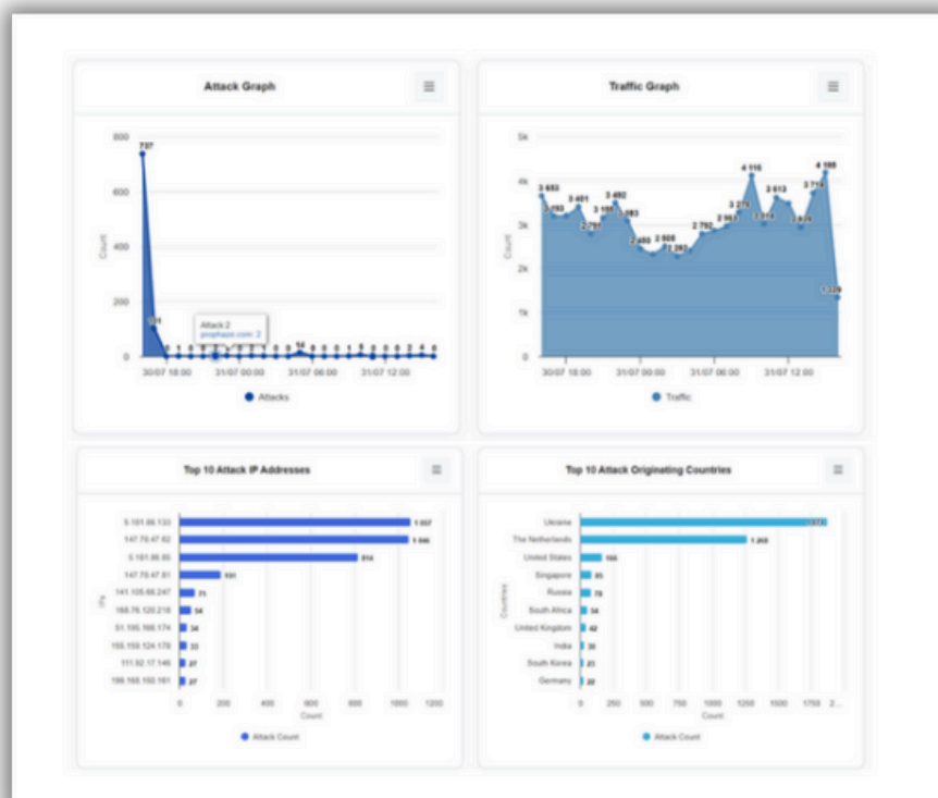
Image 6: Dashboard screenshot or mock showing traffic graphs, attack types, and top targeted endpoints.
